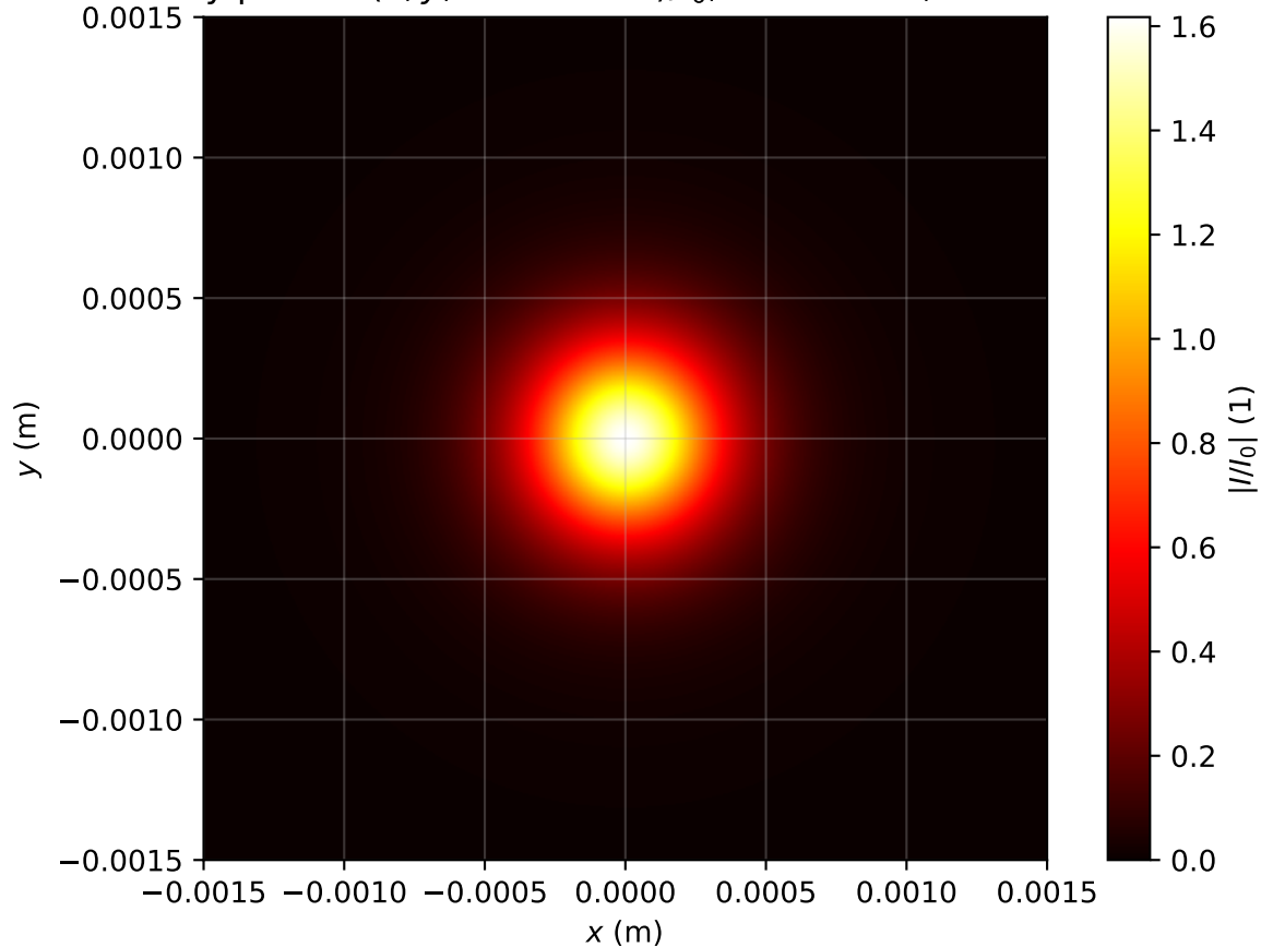
Intensity profile I(x, y, z = 2.548m)/I_0 , Pin=0.9Pcr, artificial time
